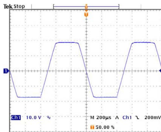
1kHz sine clipped by current limit into 250Ω load
