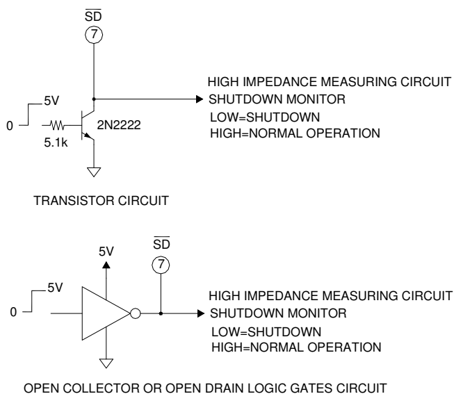
FIGURE 2. EXTERNAL SHUTDOWN
