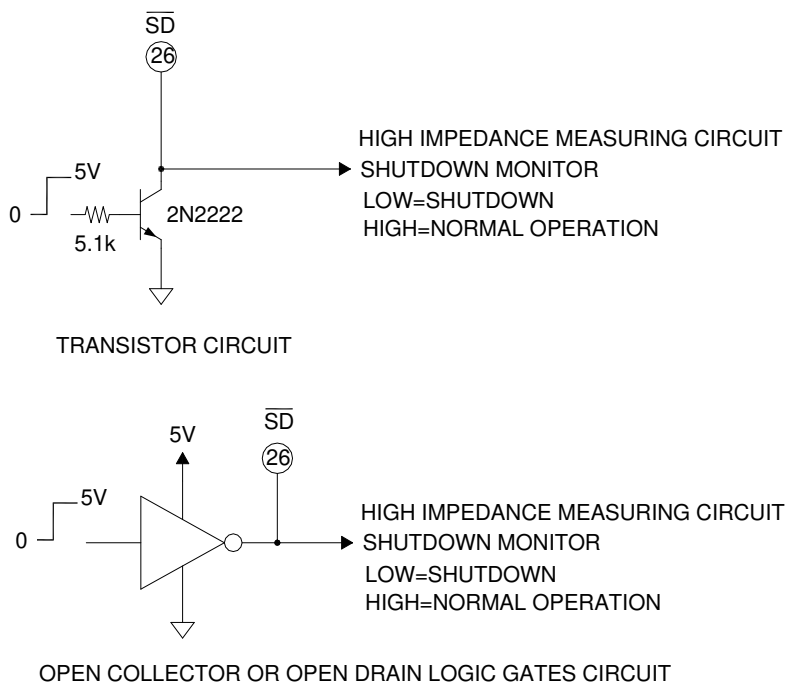
FIGURE 1. EXTERNAL SHUTDOWN WITH MONITOR
