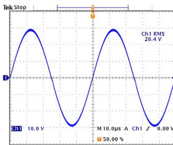
20kHz into 4 \Omega load, G=-10, Cc=100pF
