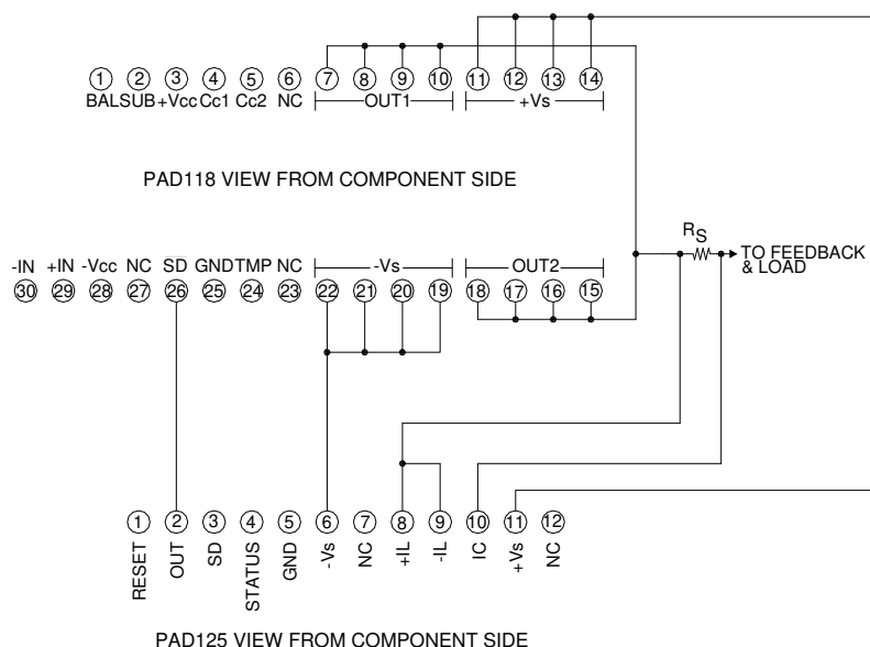
FIGURE 2. TYPICAL PAD118 CONNECTIONS TO PAD125 ACCESSORY MODULE
