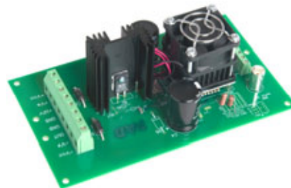
Assembled EVAL138 with amplifier installed.
