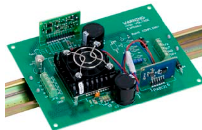
Assembled EVAL112 with amplifier installed. Optional accessory modules also installed. Optional 35mm DIN rail mounting shown.
