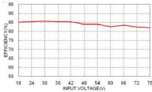
TWB3-48S5/MHIA5 Efficiency VS Input Voltage
