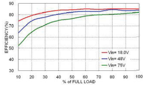
TWB3-48S5/MHIA5 Efficiency VS Output Load
