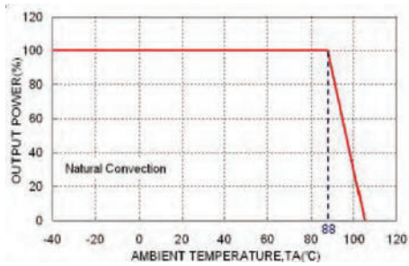
TWA6-48S5/MHIA5 Derating Curve
