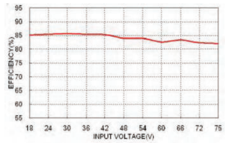
TWA3-48S5/MHIA5 Efficiency vs. Input Voltage
