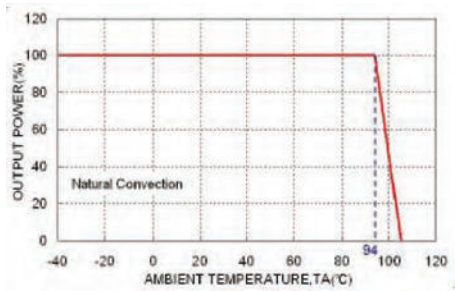
TWA3-48S5/MHIA5 Derating Curve
