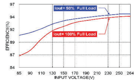
Efficiency vs. Input Voltage With forced air cooling
