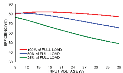
DSB(H)3-48S5 Efficiency vs. Input Voltage
