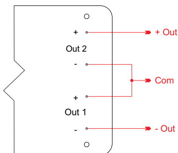
Bipolar Output
