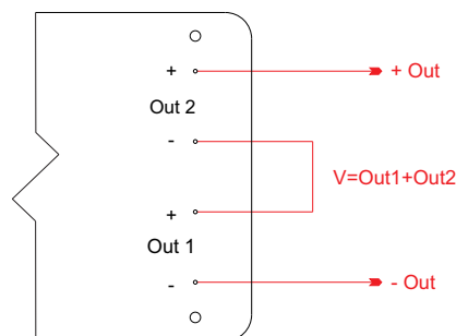
Outputs > 500Vdc
