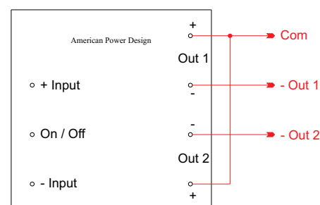
Dual Negative Output
