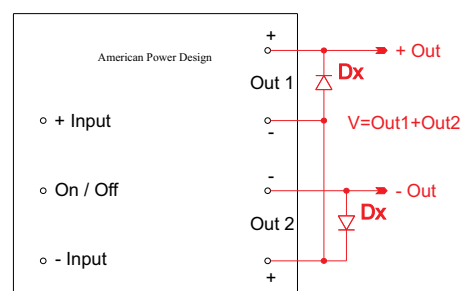
Outputs > 500Vdc
