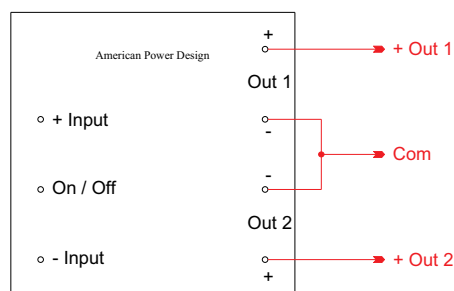
Dual Positive Output
