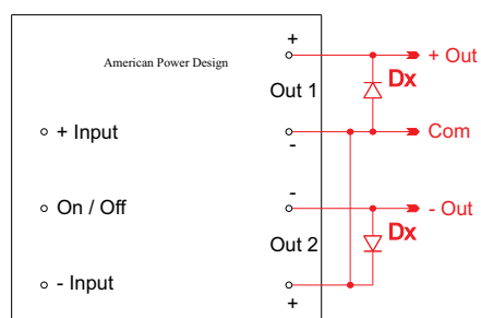
Bipolar Output
