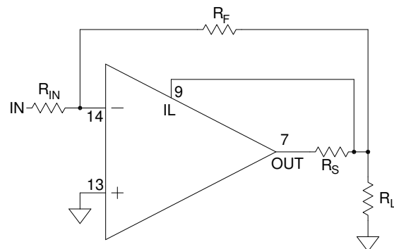
Figure 1 Current Limit
